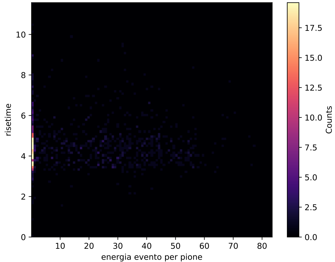
pion distribution 80.0GeV
