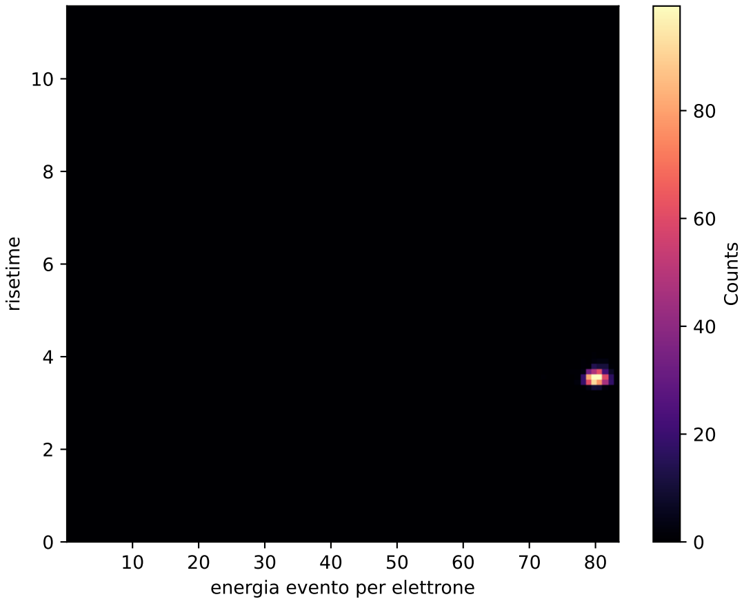
electron distribution 80.0GeV
